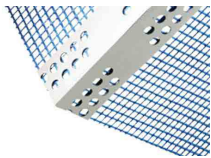
Betoncorner Alu - Angular glass fiber net with a density of 165 g/m 2 reinforced with al aluminium profile that forms a 90° angle. Used for corners, sharp edges panels.
